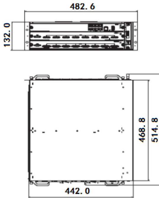
DMC8000-3U
